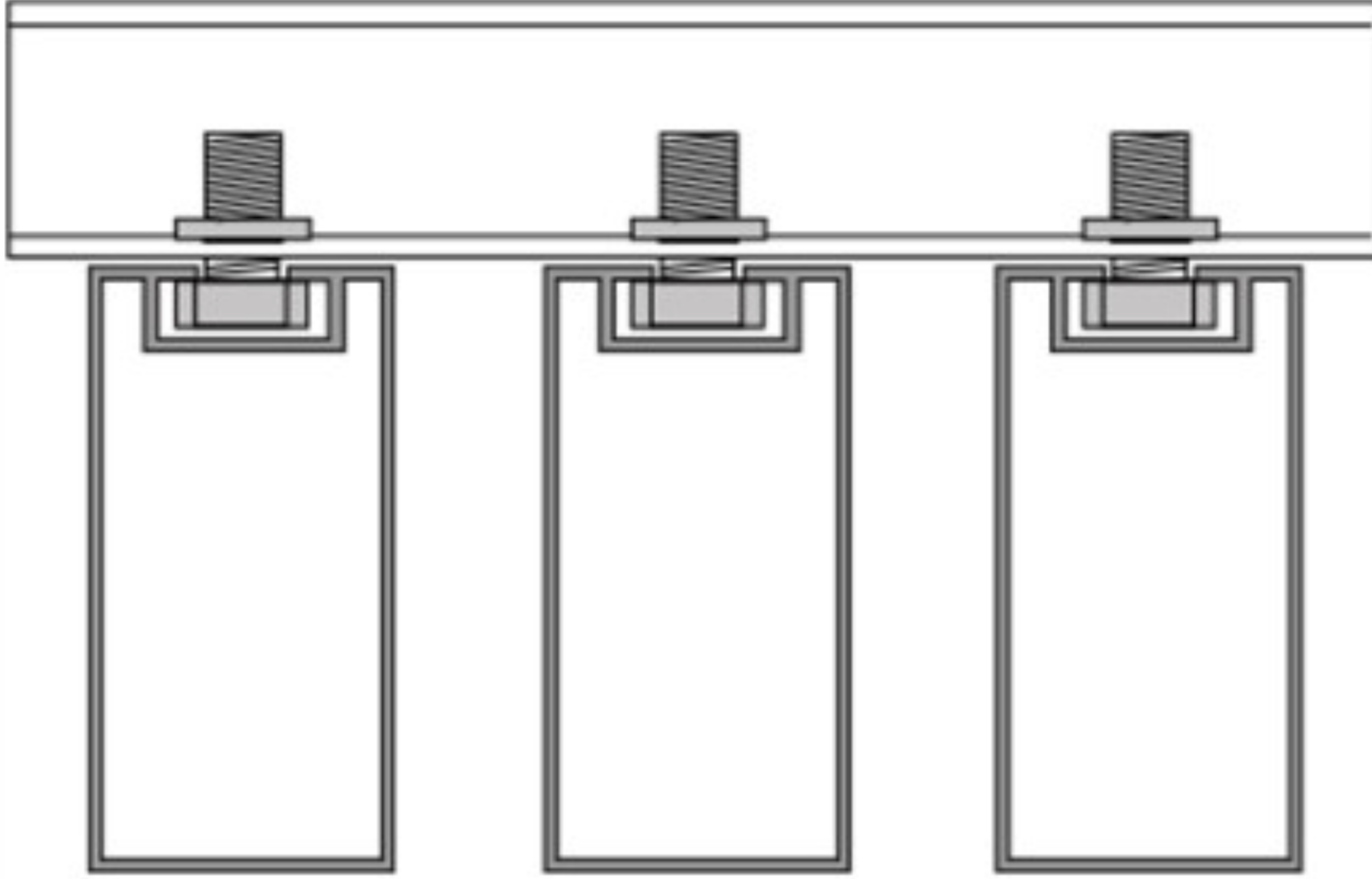
Screw linked installation
