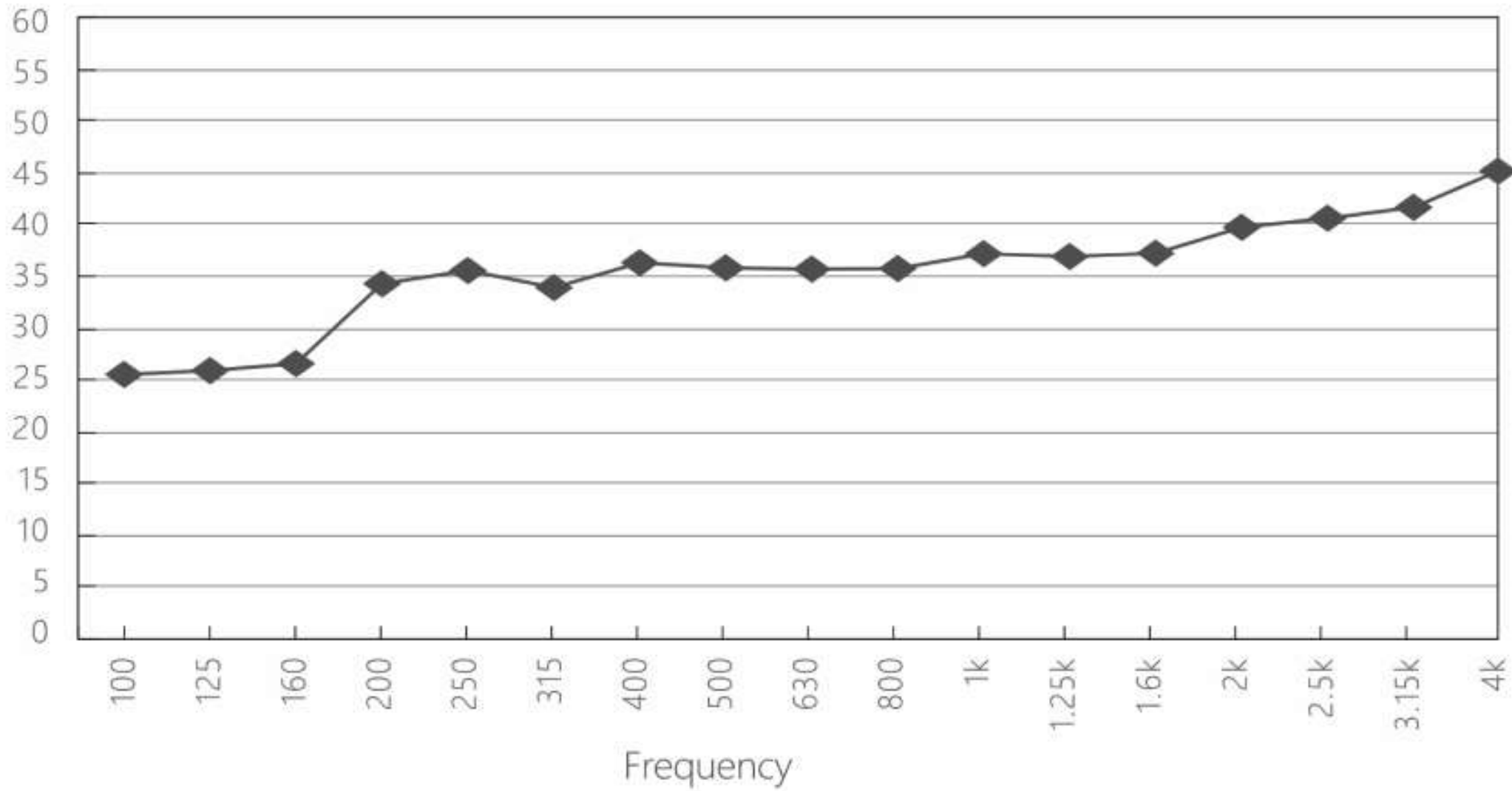
Airborne Sound Reduction Index
