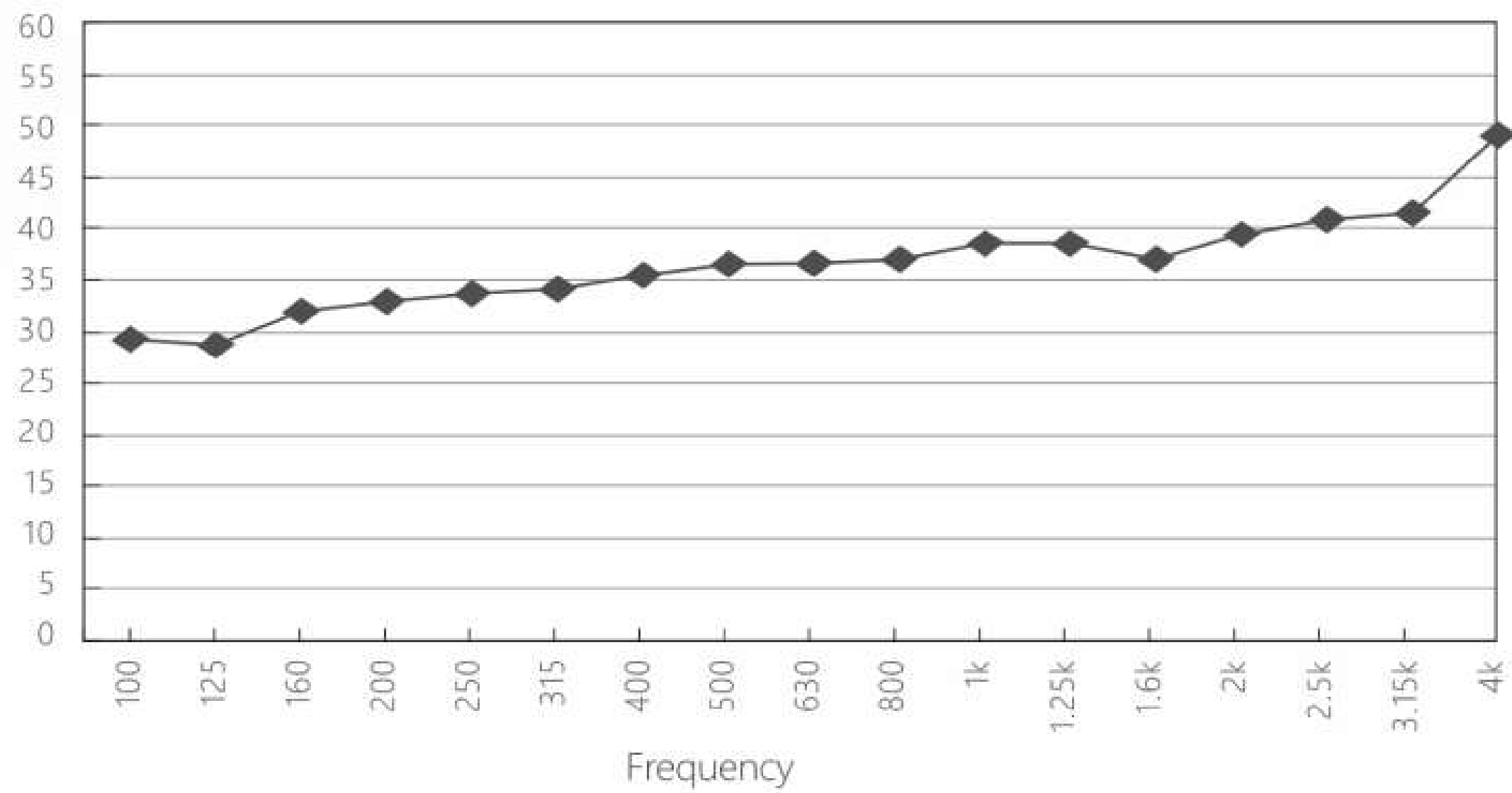
Airborne Sound Reduction Index
